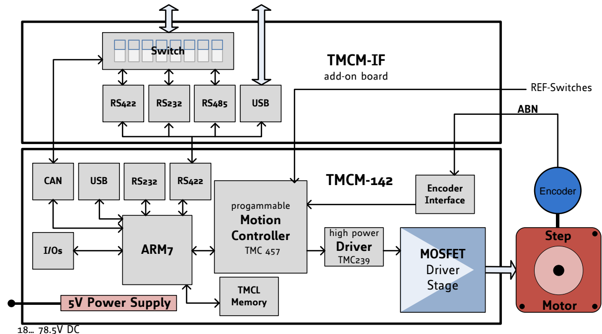
Figure 5.1: Main parts of TCM-142 with TCM-IF
